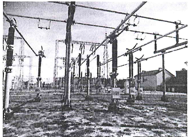
Pole 220 kV – Autotransformator AT1
