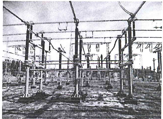
Pole 220 kV – Autotransformator AT3
