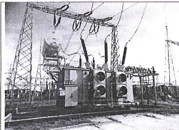
Autotransformator AT2
