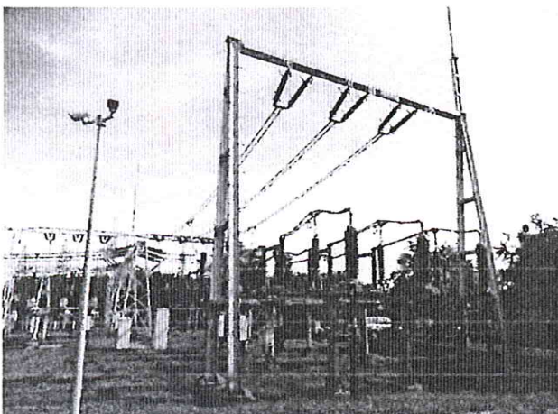
Pole 110 kV – autotransformator AT3
