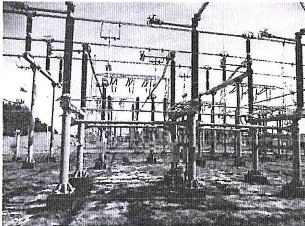
Pole 220 kV – Autotransformator AT2
